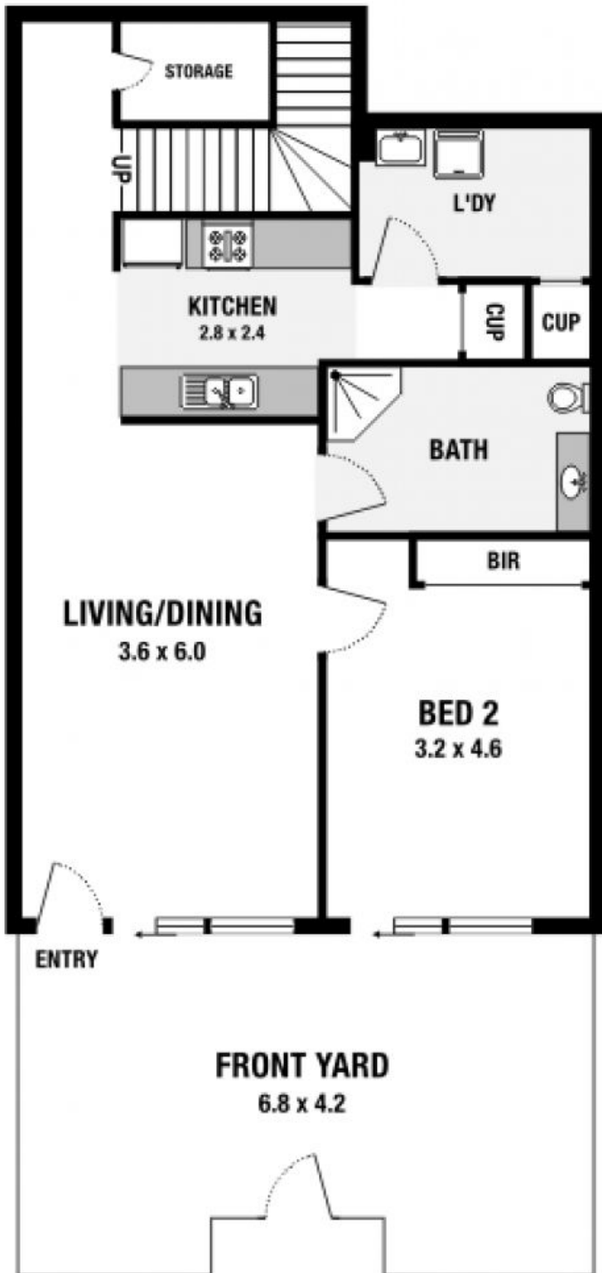
GROUND FLOOR
