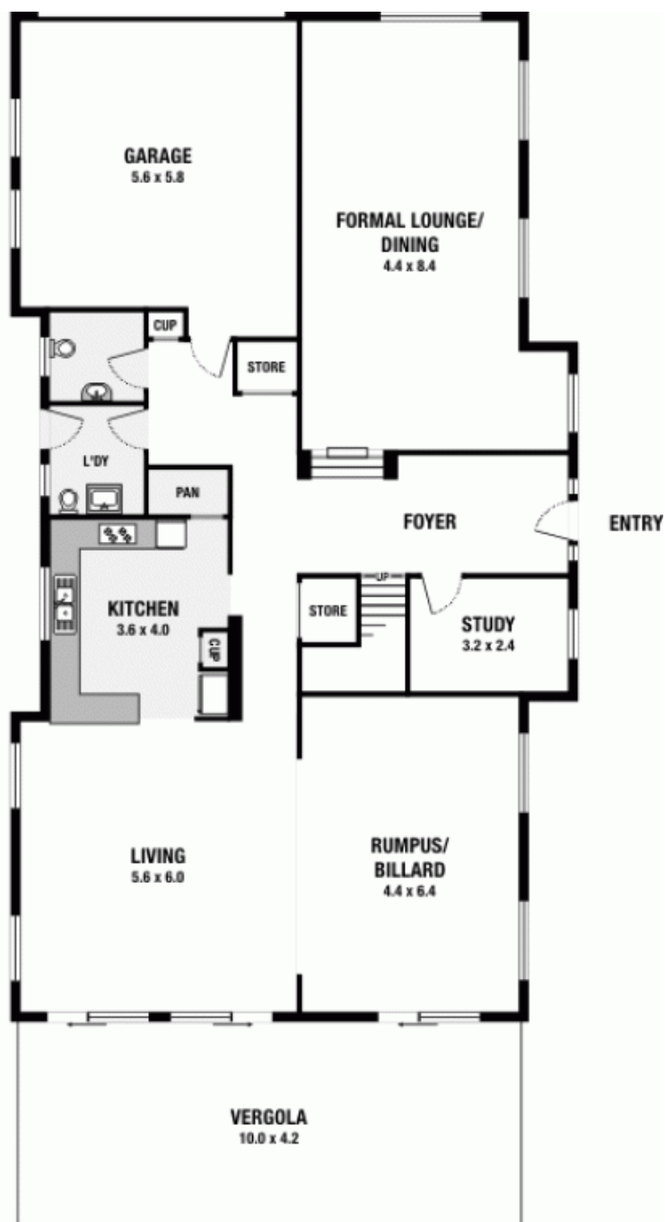
GROUND FLOOR
